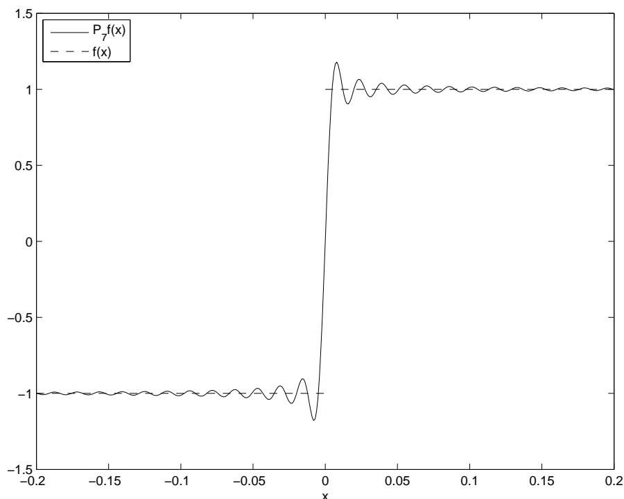
Figure 5.5.2: Graph of f(x) and its Shannon approximation for j=7
