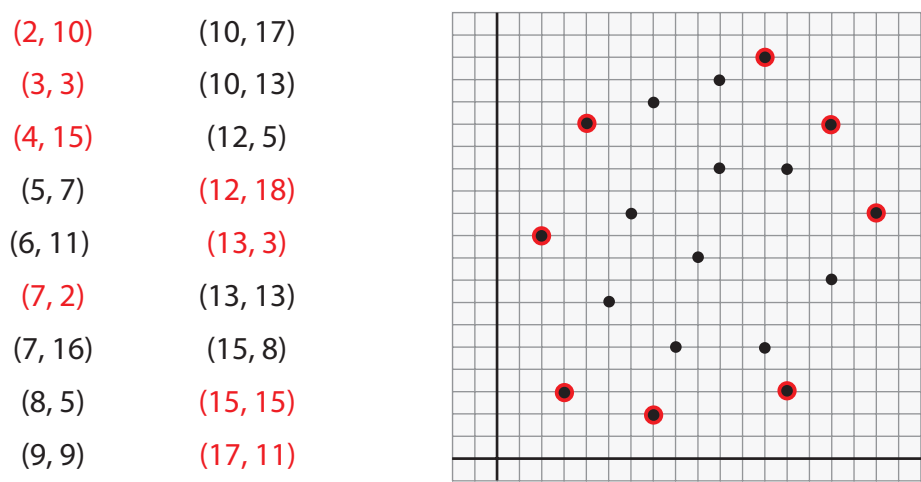
Figure 2.2. The left side lists 18 points, with the hull points colored red. The right side shows the plot of these points in the plane, again with the hull points marked.
