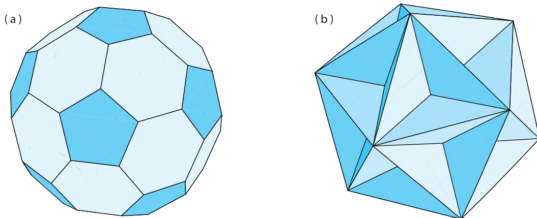
Figure 6.3. (a) Truncated icosahedron and (b) great dodecahedron.
