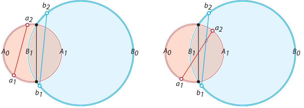
Figure 4.9. Crossing chords.
