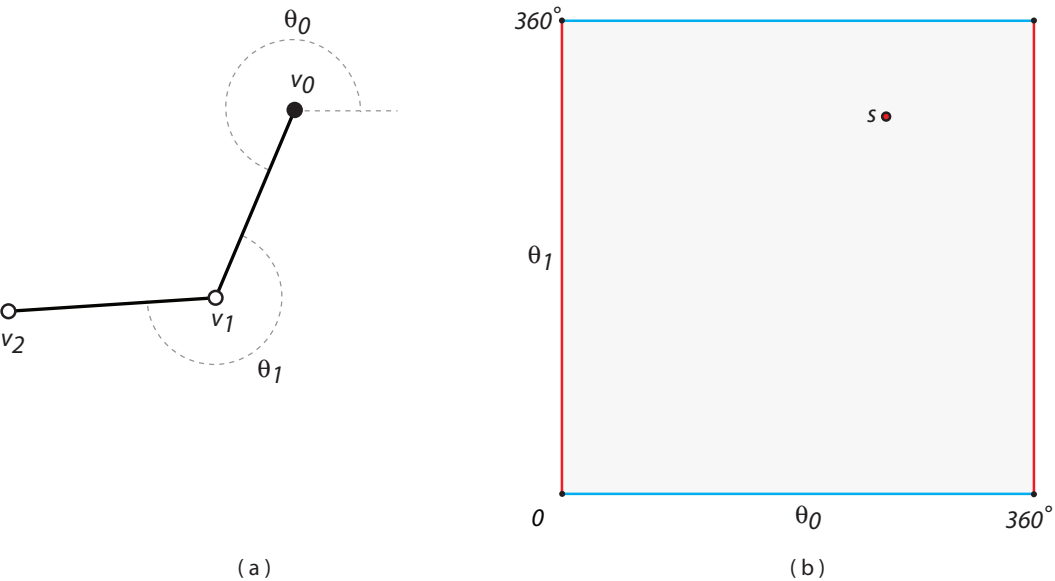
Figure 7.9. (a) A 2-link arm and (b) its configuration space.
