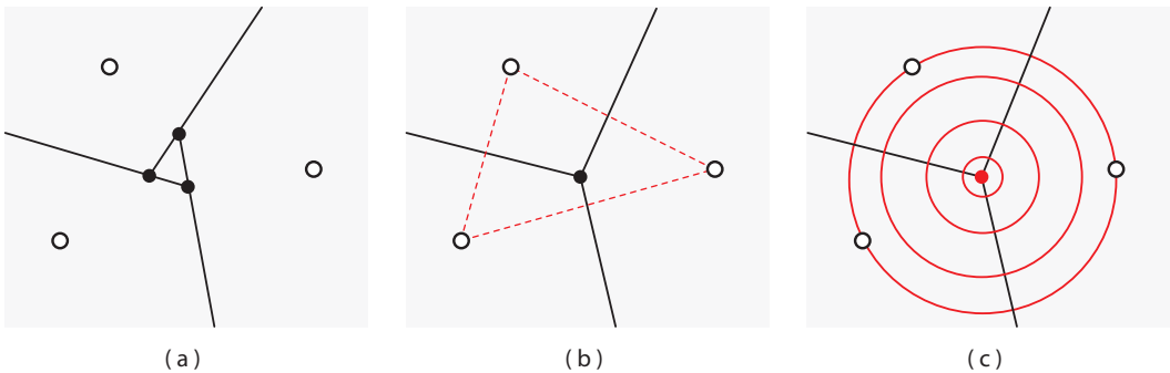
Figure 4.2. Bisectors and circumcircles with three sites.
