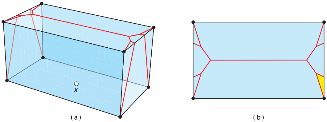
Figure 6.30. (a) The cut locus C(x) along with (b) a close-up of the top of the box.
