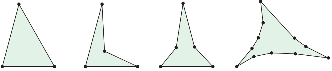
Figure 3.28. Examples of pseudotriangles.
