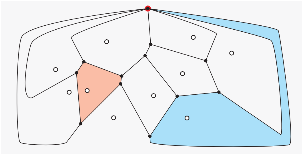
Figure 4.4. Adding an extra vertex and connecting to it the unbounded edges of Figure 4.1.
