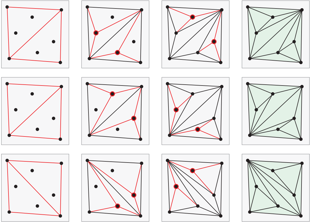
Figure 3.2. The rows show the same algorithm producing three different triangulations.
