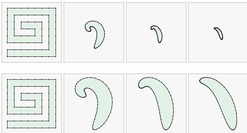
Figure 5.24. The discrete flow is applied to a spiral 64-gon with 100 iterations with \delta = 1/5 between frames. The top row is to scale whereas the bottom row shows the same sequence rescaled.
