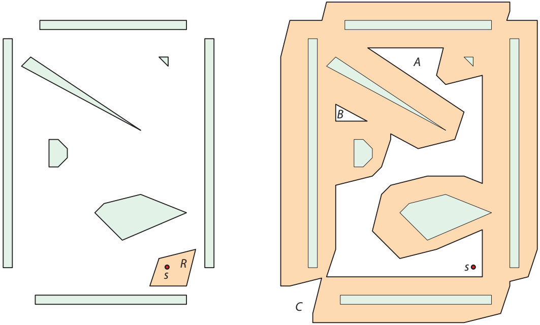
Figure 7.1. The left side shows robot R with reference point s along with polygonal obstacles. The right side shows the configuration space partitioned into three connected components A, B, C , deriving from complements of Minkowski sums with -R .
