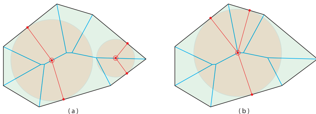
Figure 5.2. The maximal disks associated to (a) interior segments of M(P) and (b) a degree-3 vertex of M(P) .
