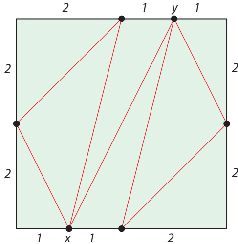
Figure 6.23. Gluing one half of the perimeter to the other half, creasing along the lines shown, results in an octahedron.
