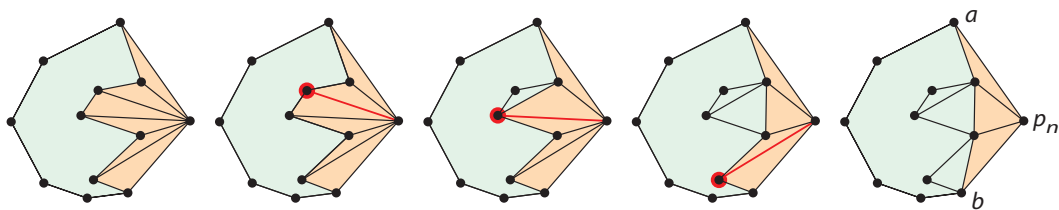
Figure 3.9. Flipping edges to obtain another triangulation.
