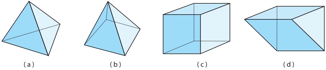
Figure 1.5. Polyhedra: (a) tetrahedron, (b) pyramid with square base, (c) cube, and (d) triangular prism.
