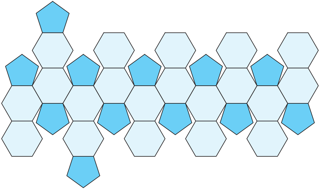
Figure 6.26. A net of the truncated icosahedron given in Figure 6.3(a).
