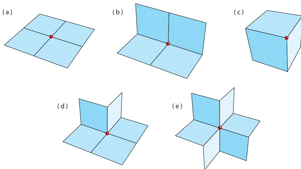
Figure 6.13. Polyhedral curvatures 0 , 0 , \pi/2 , -\pi/2 , and -\pi at the marked points, respectively.
