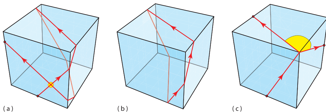
Figure 6.35. (a) Part of a self-crossing geodesic on a cube. (b) A simple closed geodesic. (c) A quasigeodesic can take many paths through a vertex.
